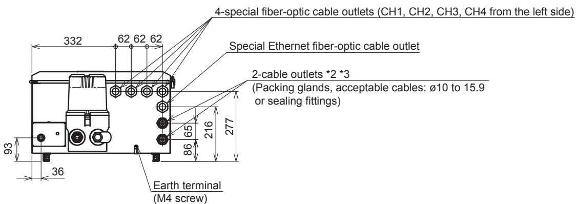
Connection: 3/4NPT Part A For NR805AG
