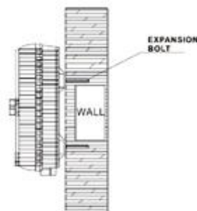
Wall mounted installation
